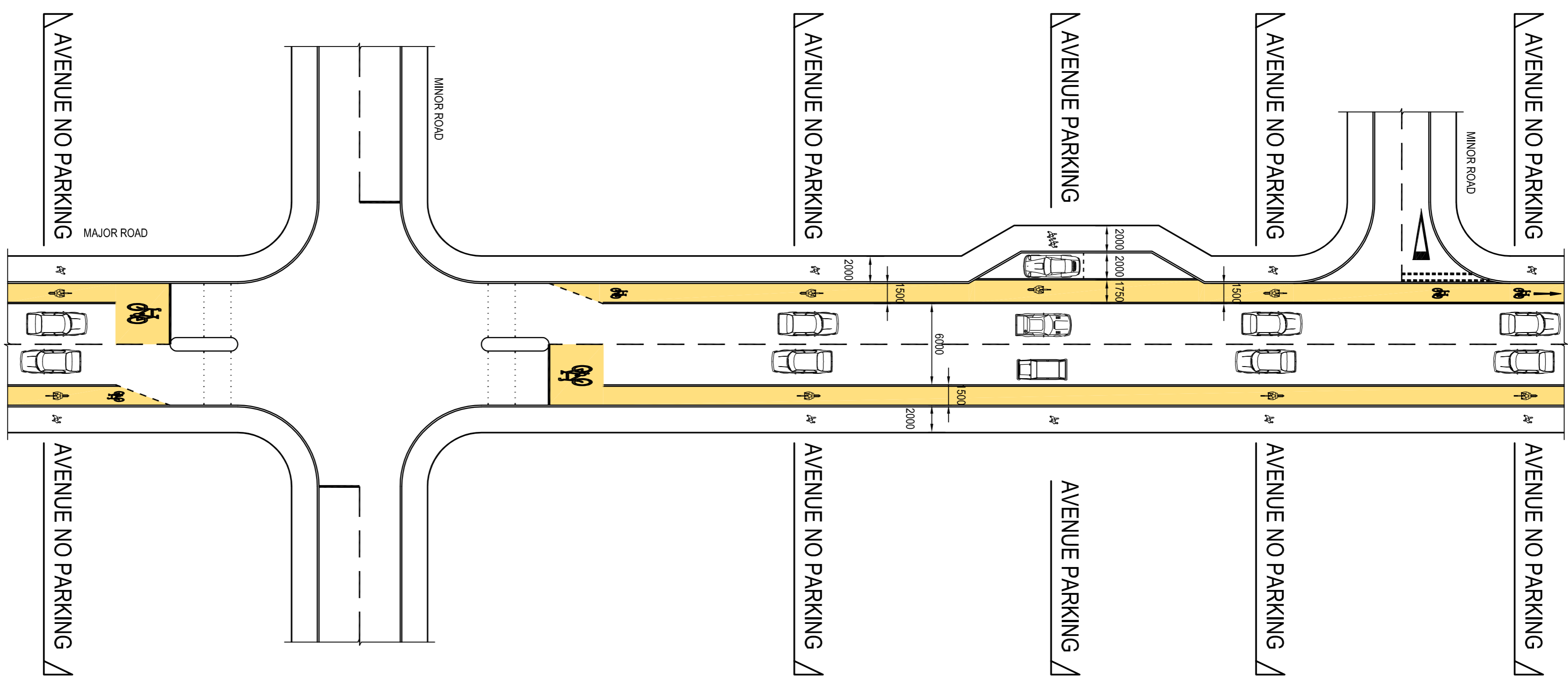
PLAN SHOWING LOCATION OF CROSS SECTIONS SCALE 1:250
