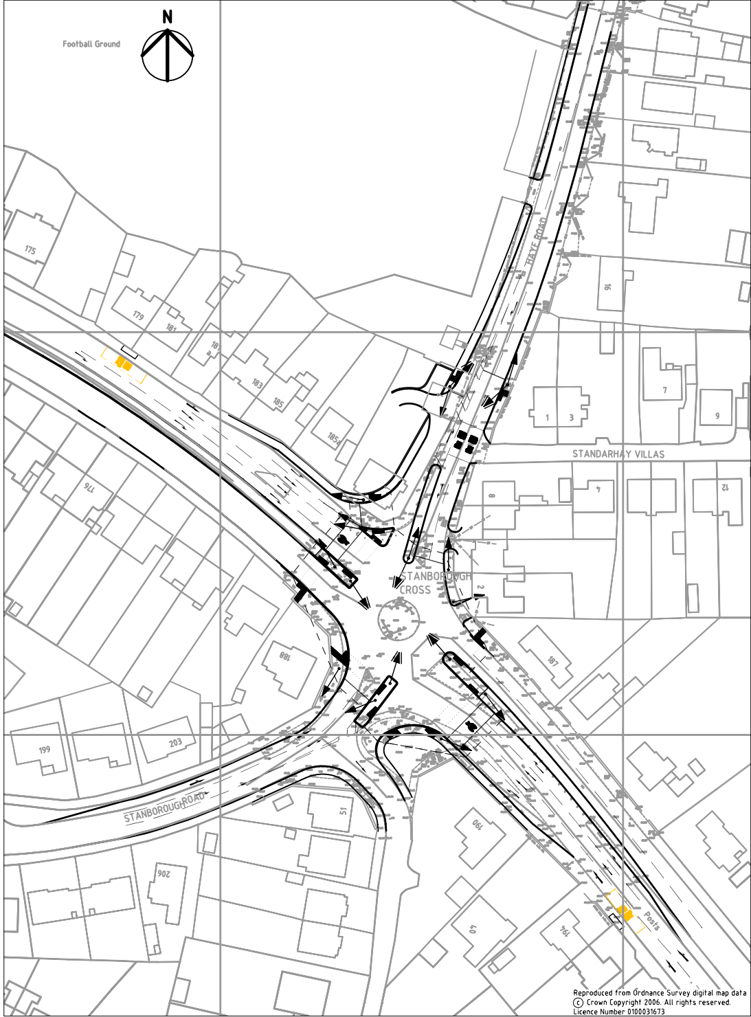
Figure 6 Stanborough Cross Proposed Layout
